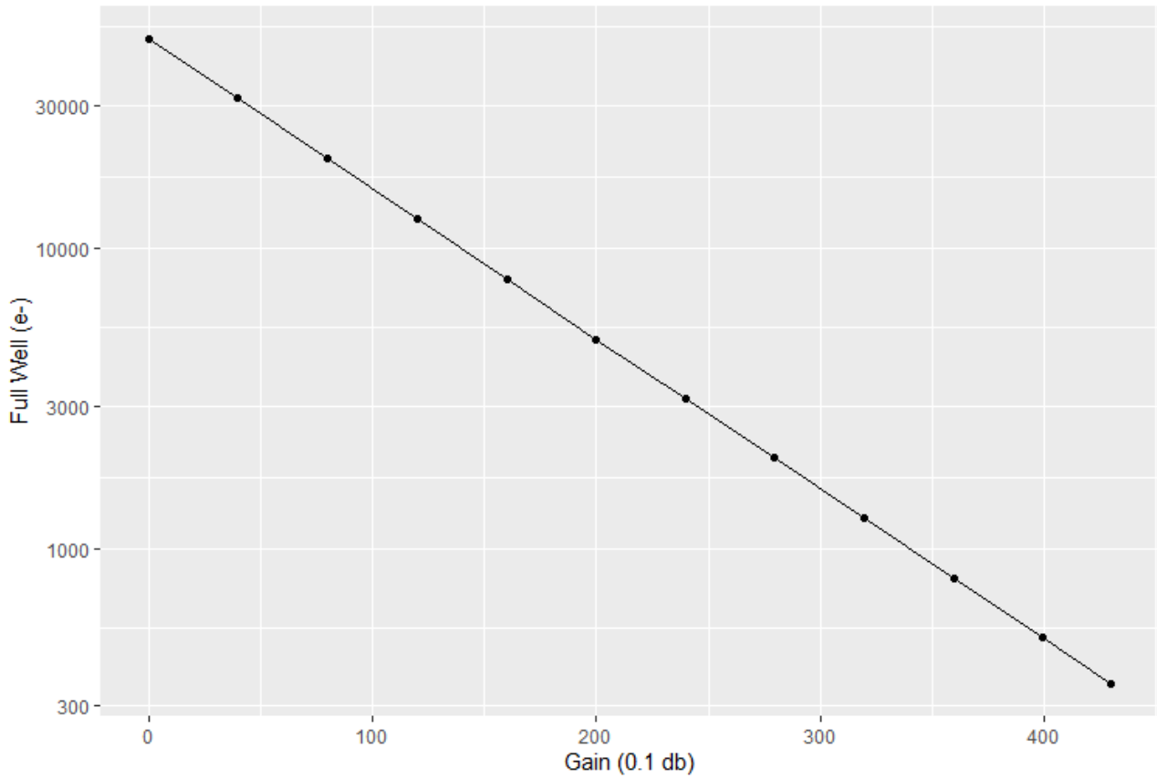
Omegon veTec 533 Gain vs Full Well (e-)
