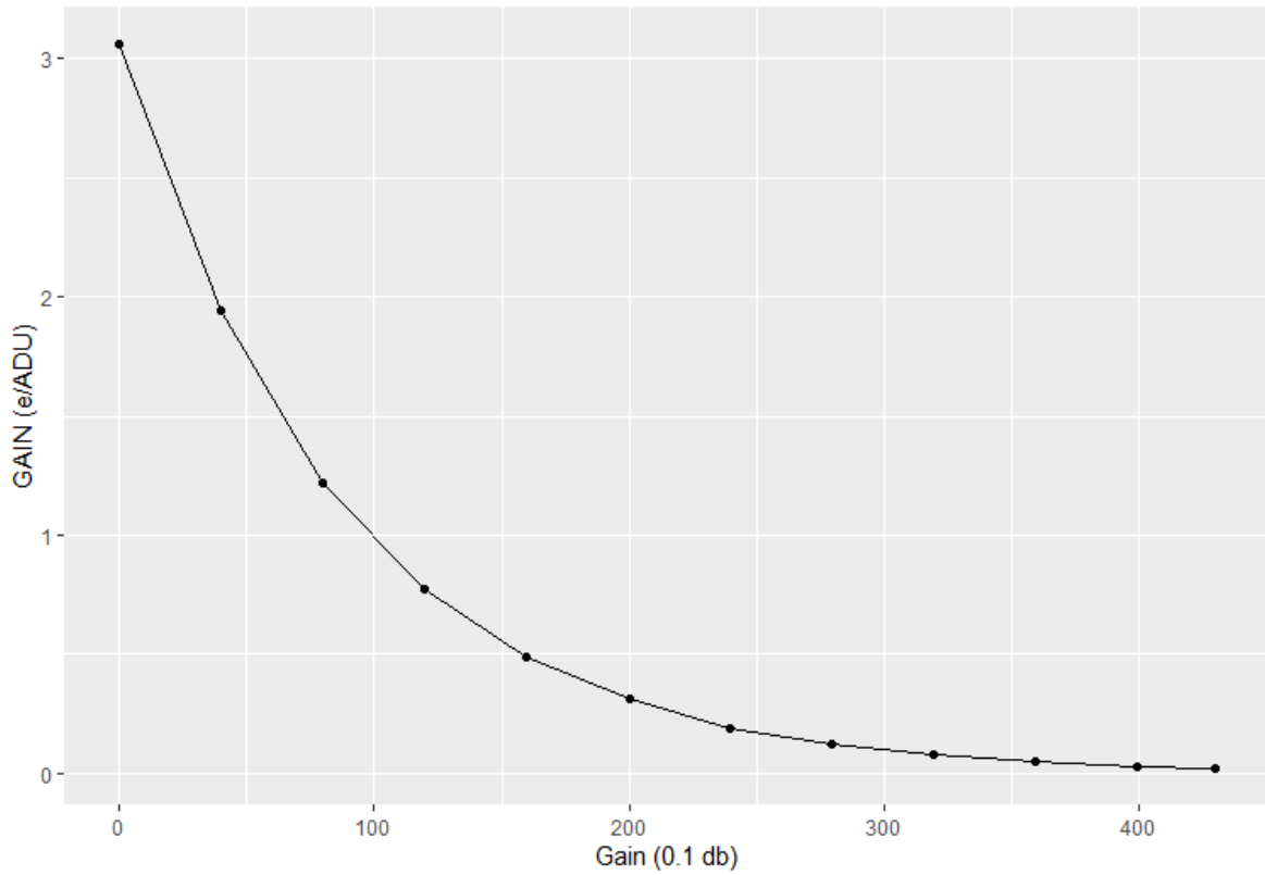
Omegon veTec 533 Gain vs GAIN(e/ADU)
