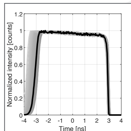
Time gating with typical 6 ns width, 350 ps rise time and 150 ps fall time. The figure shows all the gate shapes over the image sensor.
